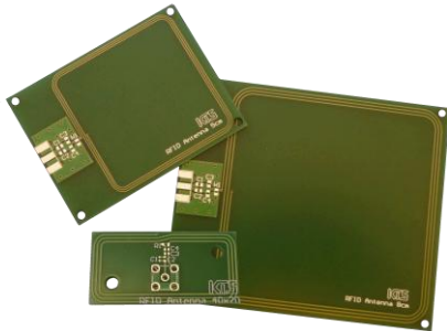
Picture 2 – Various PCB RFID Antennas
